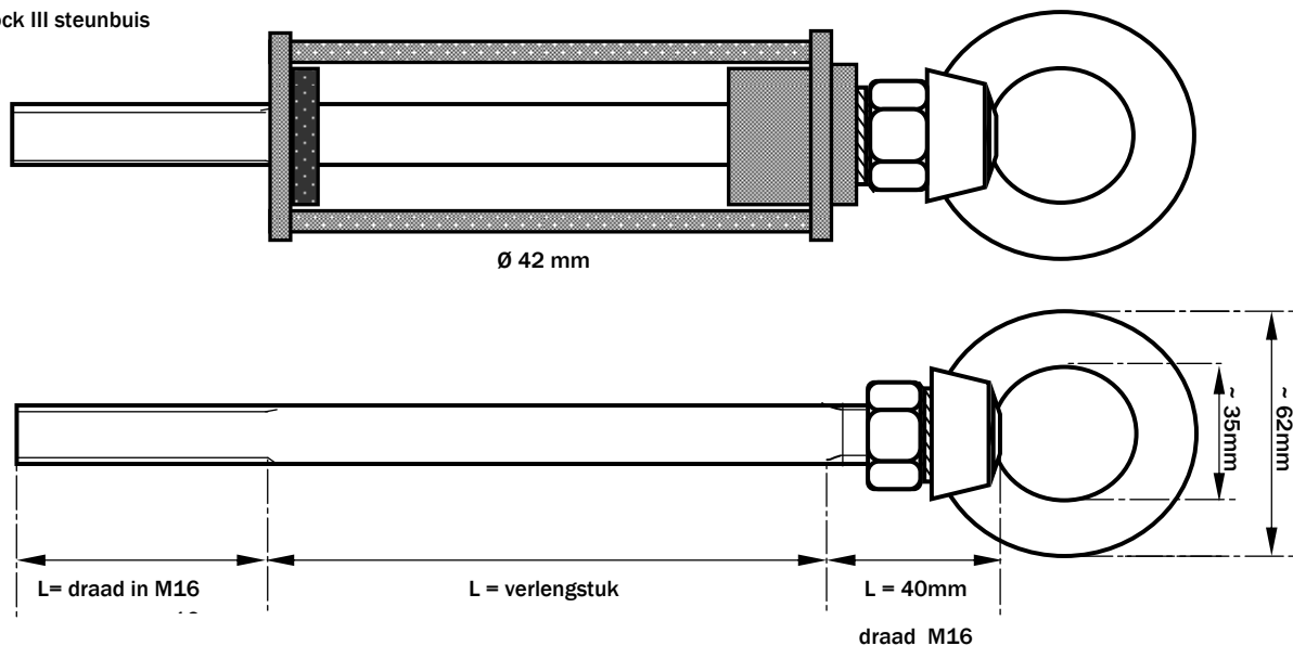
Detail ABS-Lock III steunbuis
