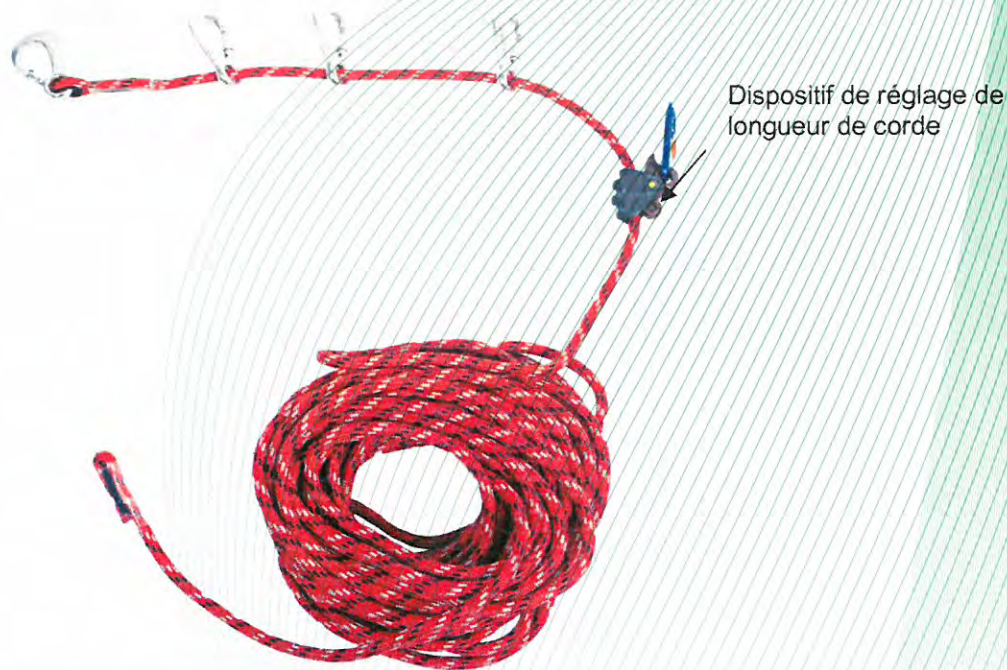
Figure 1: Dispositif d'ancrage, type: ABS ASK 8
