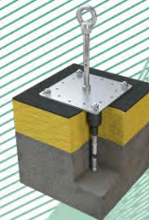
Fig. 14: Anchor device, type ABS-Lock® X-Therm
