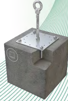
Fig. 10: Anchor device, type: ABS-Lock® X-B-A
