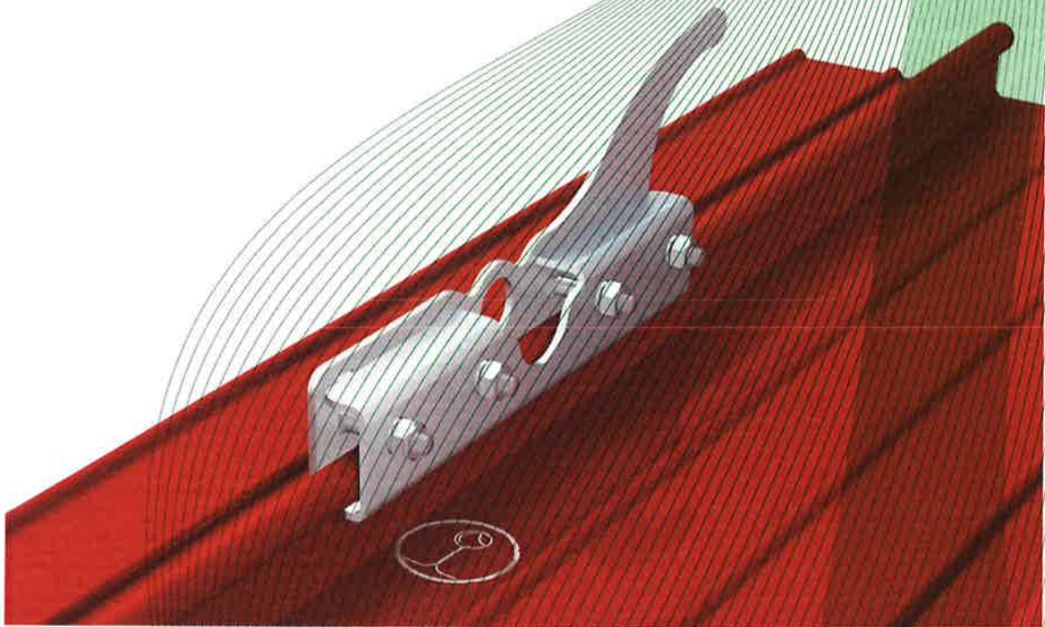
Fig. 1: Safety roof hook, type: ABS-Lock® DH06 (assembly example)
