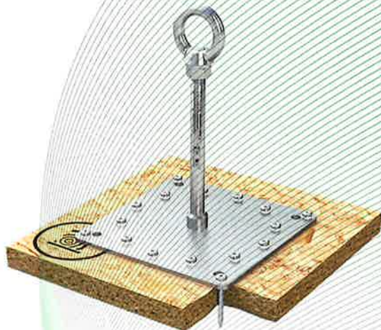
Fig. 1: Anchor device, type: ABS-Lock® X-H-14+2
